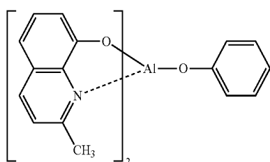
[Chemical Formula 22]
