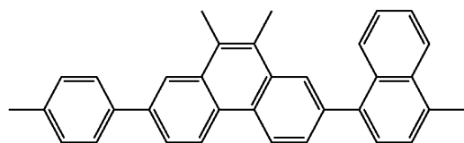
Compound A
