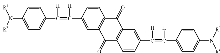
[Chemical Formula 36]
