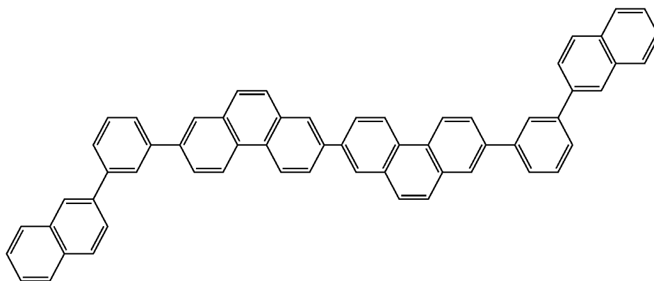
[Chemical Formula 9]
